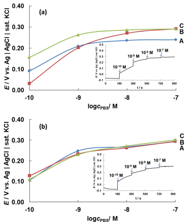
Fig. 8 OCPs ( E ) obtained for CoONPs/PBI/MWCNTs/GCE at different phosphate concentrations ( C_{\text{PBS}} = 1.0 \times 10^{-10} to 1.0 \times 10^{-7} \text{ M} ) at pH (a) 4 and (b) 7. The results of triplicate measurements are marked as A, B, and C and indicate high repeatability.
