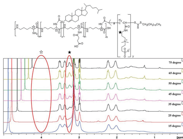
Fig. 3 Temperature dependent 1 H NMR spectra of M1 in D 2 O. Temperature increases from 15 °C (bottom curve) to 75 °C (top curve) in steps of 10 °C.
