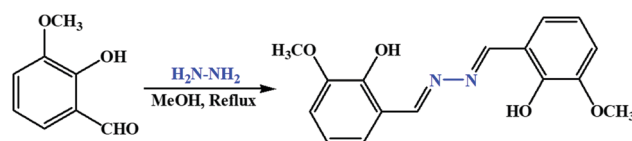
Scheme 1 Synthesis of the probe H 2 L.
