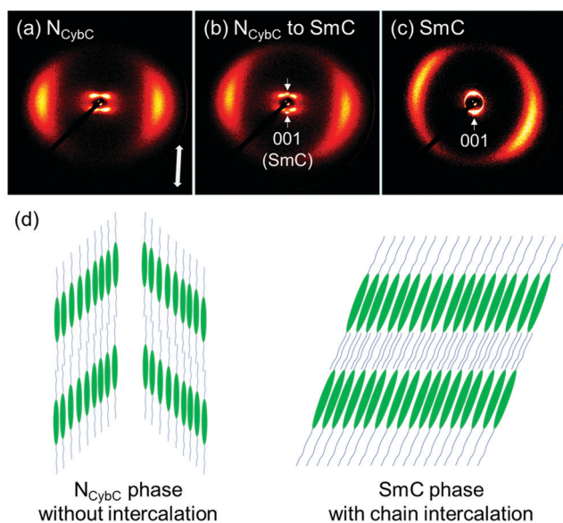
Fig. 6 2D XRD patterns of SO8 (a) in the cybotactic N ( N_{\text{Cybc}} ) phase with a tilted SmC cluster ( N_{\text{Cybc}} phase) at 140 °C, (b) during the N–SmC phase transition at 130 °C, and (c) in the SmC phase at 120 °C. (d) Schematic packing models of the N_{\text{Cybc}} and SmC phases.
