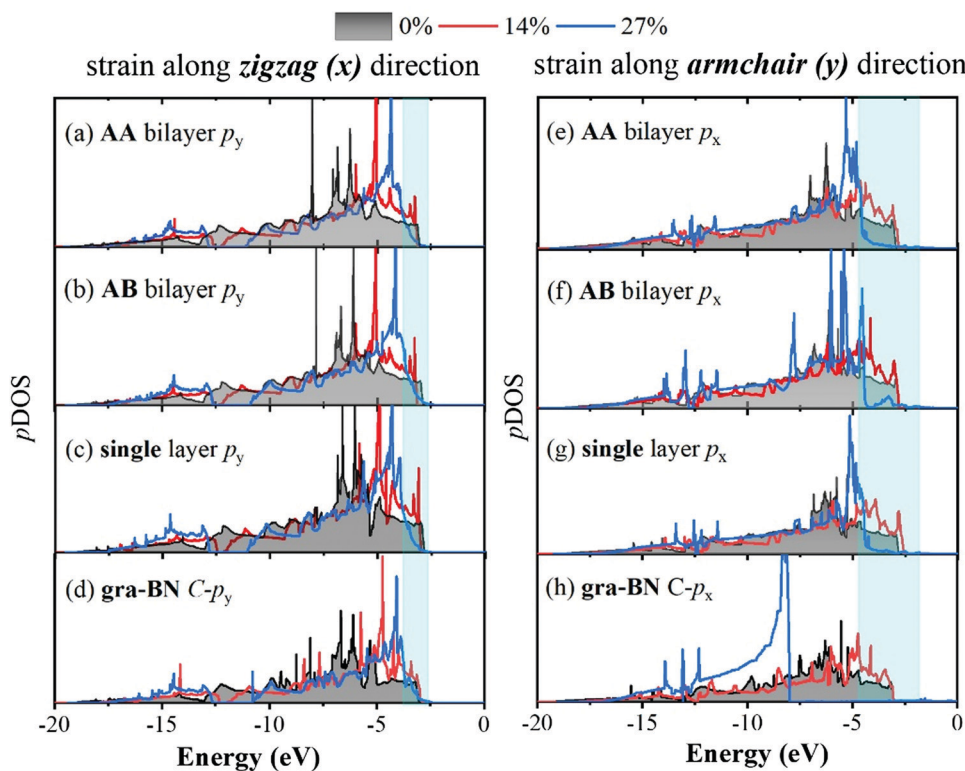
Fig. 6 (a–d) The evolution of p_y when strain is applied along the zigzag direction ( x ). (e–h) The evolution of p_x when the strain is applied along the armchair direction ( y ). (a and e), (b and f), (c and g), (d and h) illustrate the situation for the AA bilayer, AB bilayer, single-layer graphene and gra-BN, respectively. The cyan border highlights the key evolution around the valence band maximum.
