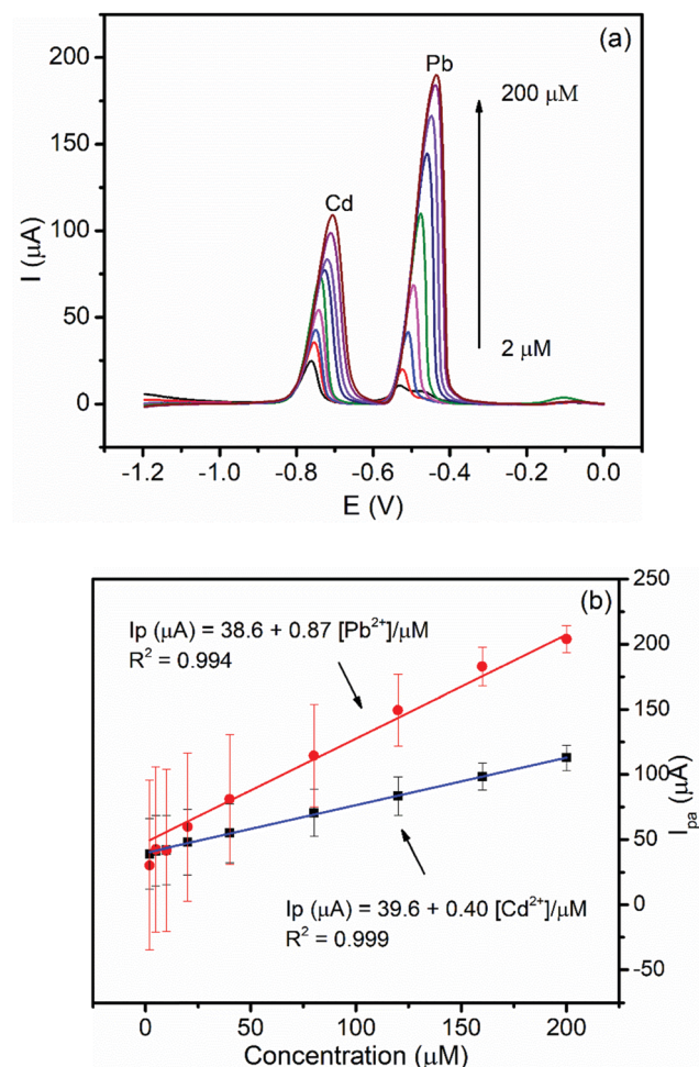
Fig. 7 (a) Corrected curves for the blank DPSV of the BFO/CPE in PH 4.5 ABS containing different equimolar mixtures of Pb(II) and Cd(II) (2, 5, 10, 20, 40, 80, 120, 160, and 200 \mu M, respectively) at E_{acc} -1.2 V and t_{acc} 180 s. (b) Calibration plot of the concentrations of Pb(II) (red line) and Cd(II) (blue line) vs. the peak current.
