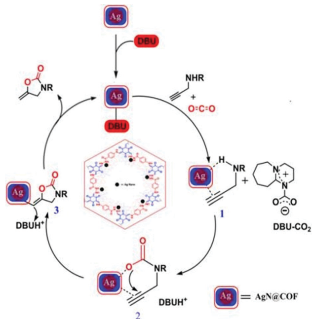
Scheme 36 The reaction mechanism for 2-oxazolidinone synthesis using the synthesized AgNPs@COF material. Reproduced with permission from ref. 61; copyright: 2020, ChemNanoMat.
