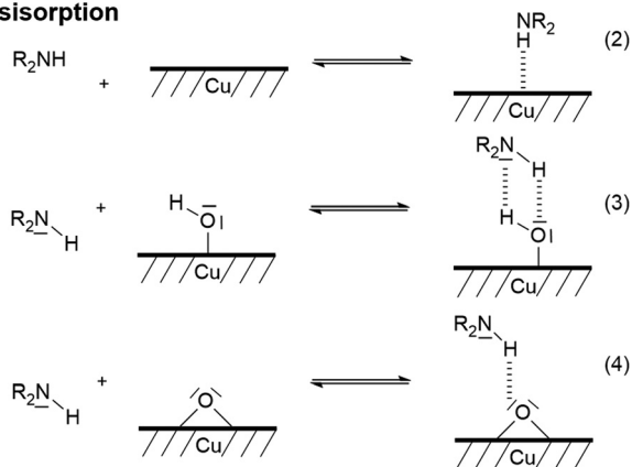
Scheme 3 Suggested bonding states of secondary amines on copper surfaces according to the literature. 91
