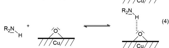
Scheme 3 Suggested bonding states of secondary amines on copper surfaces according to the literature. 91
