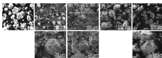
Fig. 5 SEM micrographs of phenolic resin–silica hybrid material-coated ttPAN particles obtained by DABCO-catalysed surface twin polymerisation using 25 wt% (b and c), 50 wt% (d and e), 70 wt% (f), and 88 wt% (g and h) of TM on the ttPAN substrate compared to that of the starting ttPAN material (a).
