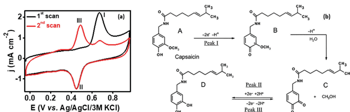
Fig. 2 (a) Two successive cyclic voltammograms in the presence of 100 \mu\text{M} capsaicin at a scan rate of 25 \text{mV s}^{-1} showing electrochemical oxidation of capsaicin; (b) mechanism showing the reaction pathway of electrochemical oxidation of capsaicin. 40,41
