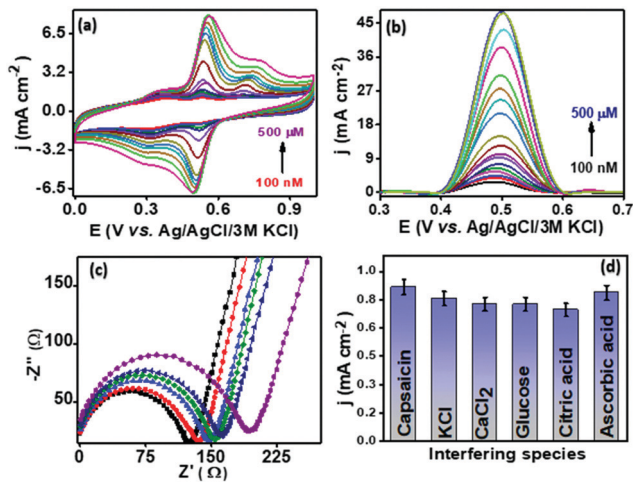
Fig. 4 (a) CV, (b) SWV and (c) EIS response of the PMF/OCNT modified electrode in 50 \text{ mM} BR buffer at various conc. of capsaicin; (d) bar diagram representing the current density w.r.t. interferences at a 100 \mu\text{M} concentration of capsaicin.
