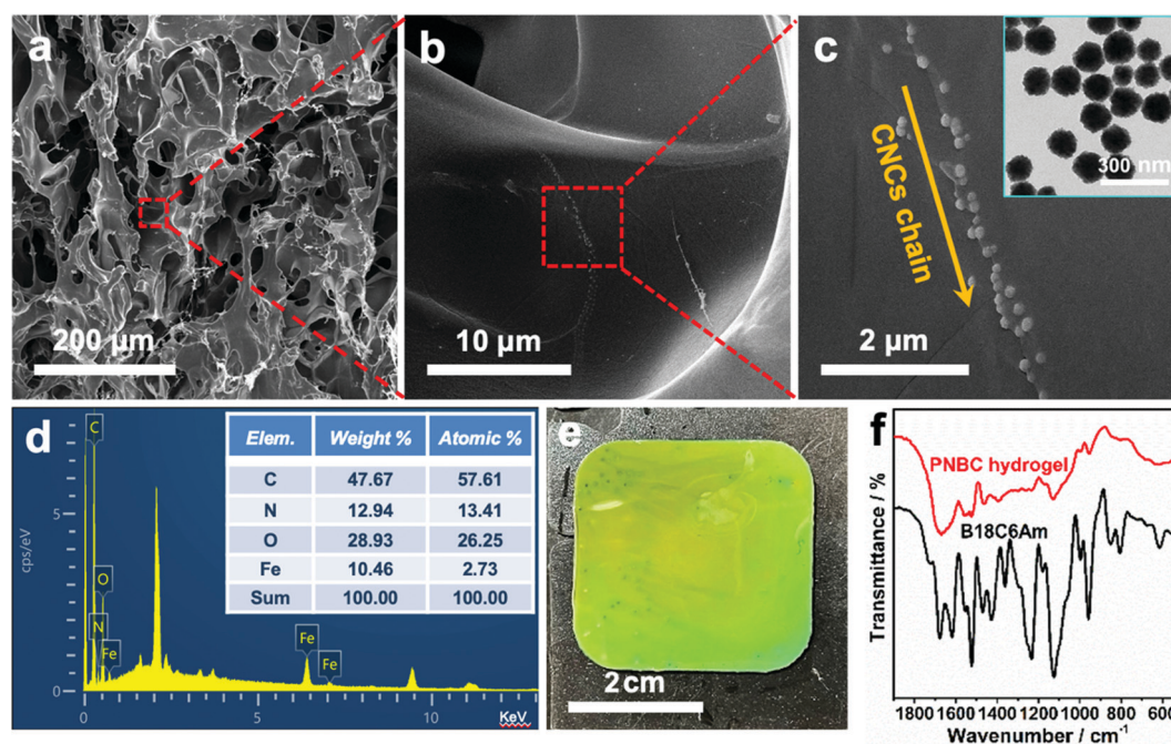
Fig. 2 Characterization of the PNBC photonic hydrogel sensor. (a) Cross-sectional SEM image of the PNBC hydrogel and (b) and (c) the 1D chainlike structure of the superparamagnetic \text{Fe}_3\text{O}_4 CNCs within the PNBC hydrogel. The inset in (c) shows the TEM image of the as-synthesized \text{Fe}_3\text{O}_4 CNCs. (d) EDS spectrum and elemental analysis of the PNBC hydrogel for the red dashed box in (a). (e) Photograph of the PNBC hydrogel. (f) FT-IR spectra of the PNBC hydrogel and B18C6Am monomer.
