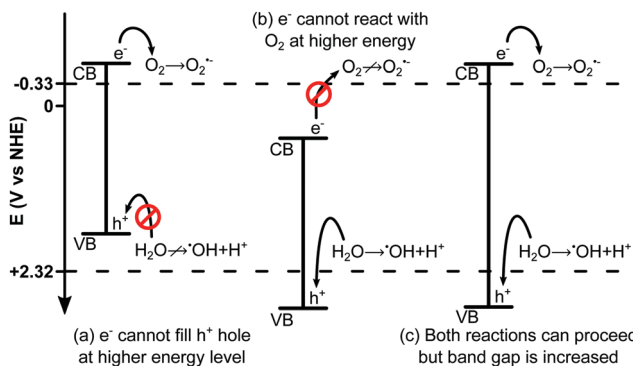
Fig. 6 Schematic illustration of redox potential for \bullet OH and O_2^{\bullet -} showing (a) a semiconductor with sufficiently negative CB to allow O_2 + e^- , but VB too negative to allow H_2O \rightarrow \bullet OH + H^+ as H_2O cannot donate an electron to fill the more negative hole in the VB of the semiconductor. (b) A semiconductor with sufficiently positive VB such that H_2O may donate an electron to fill the hole, however the CB is too positive meaning O_2 cannot accept e^- . (c) A semiconductor with both a sufficiently negative CB, and a sufficiently positive VB. This semiconductor would be capable of facilitating both reactions but has an increased band gap, limiting its solar spectrum adsorption range. Heterojunctions (Fig. 7) can be used to reduce this band gap whilst maintaining the redox potentials. Figure is for illustrative purposes only and is not drawn to scale.
