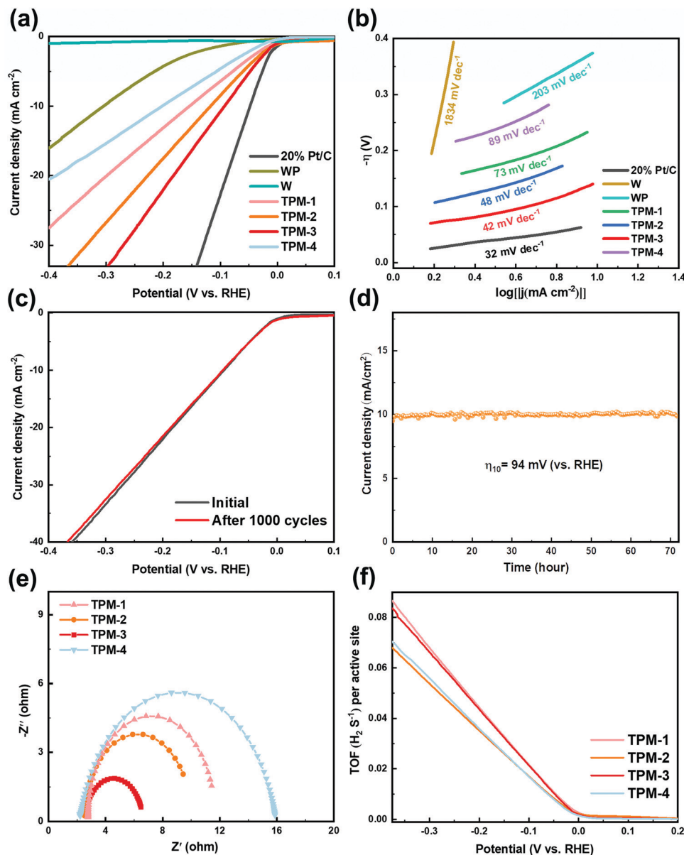
Fig. 5 The electrocatalytic HER performance of TPM-1, TPM-2, TPM-3, TPM-4, W, WP, as well as 20 wt% Pt/C in acid (0.5 M H 2 SO 4 ) media. (a) Polarization curves; (b) corresponding Tafel slope diagrams; (c) LSV curves before and after 1000 CV cycles for TPM-3; (d) i - t curve at an overpotential of 94 mV for TPM-3; (e) EIS curves and (f) TOF profiles of the TPMs.
