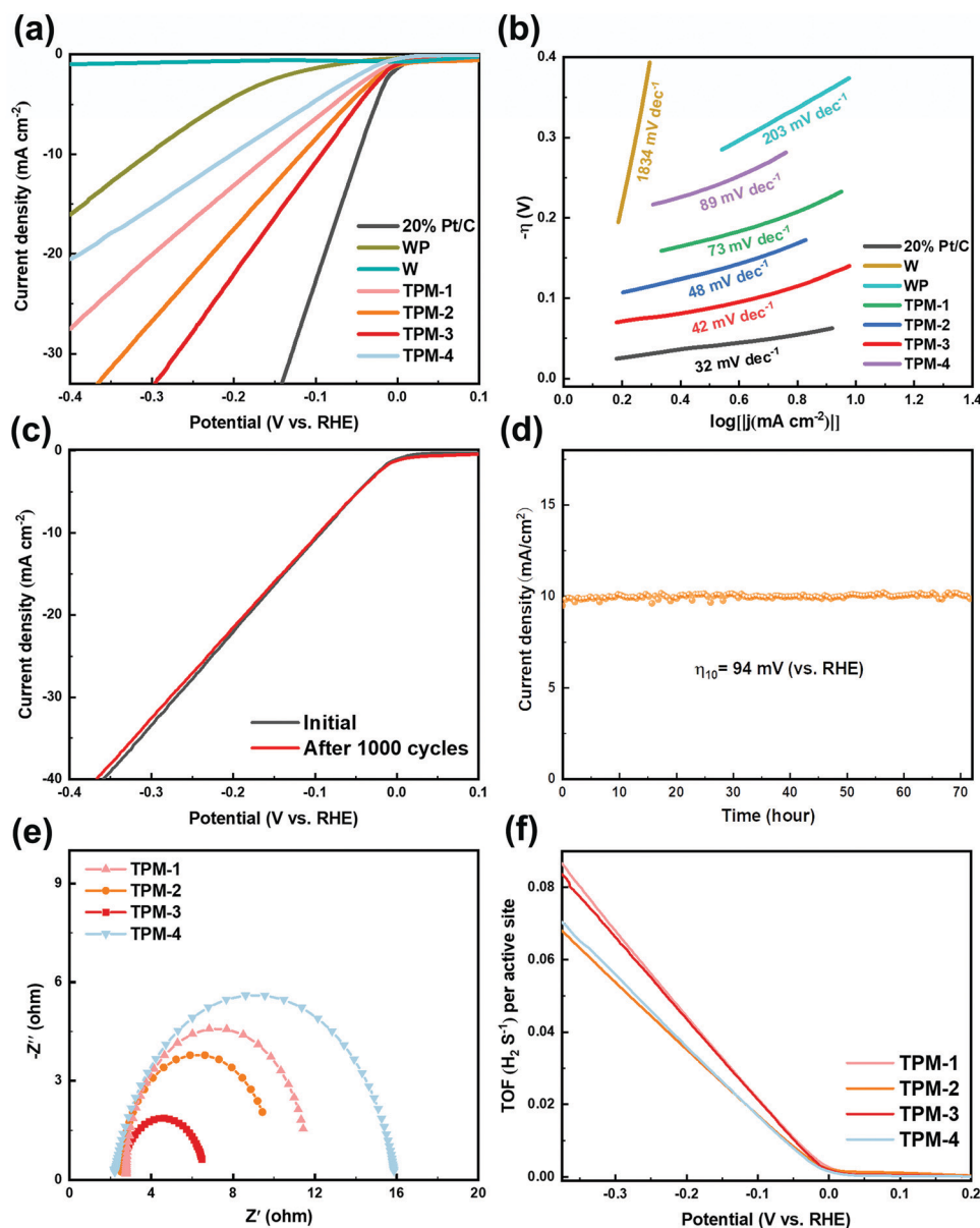
Fig. 5 The electrocatalytic HER performance of TPM-1, TPM-2, TPM-3, TPM-4, W, WP, as well as 20 wt% Pt/C in acid (0.5 M \text{H}_2\text{SO}_4 ) media. (a) Polarization curves; (b) corresponding Tafel slope diagrams; (c) LSV curves before and after 1000 CV cycles for TPM-3; (d) i - t curve at an overpotential of 94 mV for TPM-3; (e) EIS curves and (f) TOF profiles of the TPMs.
