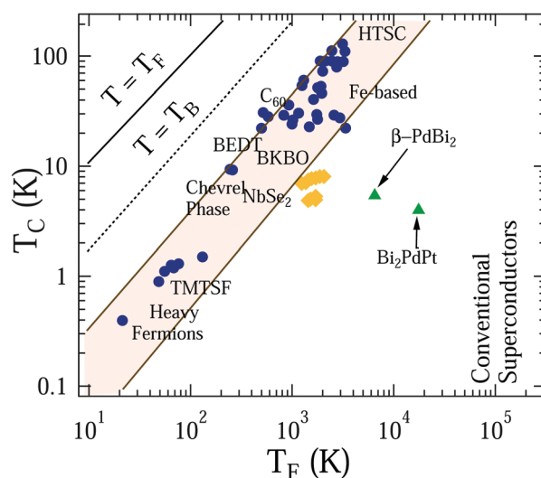
Fig. 6 Uemura plot showing the superconducting transition temperature T_C vs. the effective Fermi temperature T_F for Bi 2 PdPt with \beta -PdBi 2 , shown as solid green triangles. Other data points represent the different families of superconductors together with the shaded region representing the families of unconventional superconductors. The dashed line corresponds to the Bose–Einstein condensation temperature T_B .
