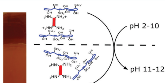
Fig. 4 (Top) UV-Vis absorption spectra of NaCS/BBY films in response to change in pH. Between pH 2–10 the \pi \rightarrow \pi^* transition absorption band is at 450 nm and at pH 11–12 there is significant broadening of the absorption band to 385–490 nm. (Bottom) Image of the film showing colour change from red (pH 2–10) to orange (pH 11–12) and a schematic of the proposed molecular changes which occur in response to change in pH.
