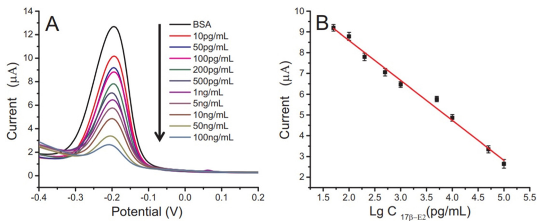
Fig. 12 (A) Differential pulse voltammetry of different concentrations of 17\beta\text{-E}_2 . (B) Microfluidic paper-based immunodevice calibration curve towards 17\beta\text{-E}_2 . Reproduced from Wang et al. (2018). 131
