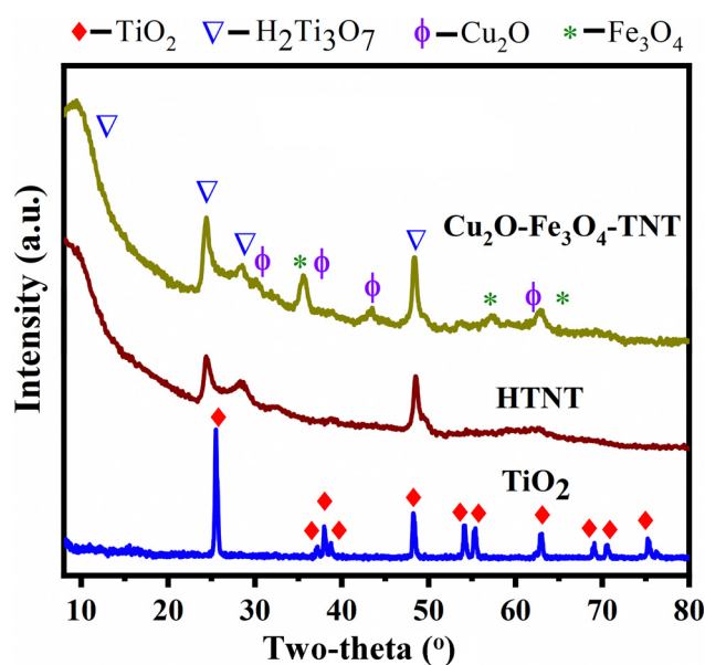
Fig. 1 XRD patterns of \text{TiO}_2 , TNT, and \text{Cu}_2\text{O}-\text{Fe}_3\text{O}_4@\text{TNT} .
