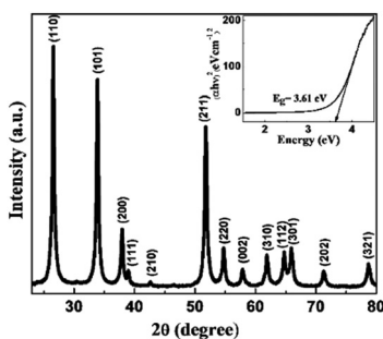
Fig. 3 X-Ray diffractogram of SnO 2 fab-fracs showing peaks corresponding to different Miller indices. The inset shows the bandgap of 3.61 eV as estimated from Tauc plot. Reprinted by permission from Springer Nature Customer Service Centre GmbH: Springer, Journal of Sol–Gel Science and Technology, Large-scale growth of tin oxide fabricated fractals, Vishal Kamathe and Rupali Nagar, Copyright (2022) Springer Nature Switzerland AG, Part of Springer Nature. 20
