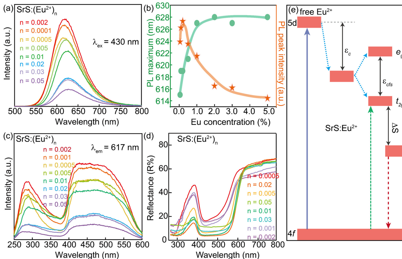
Fig. 2 (a) PL spectra of \text{SrS}:(\text{Eu}^{2+})_n under \lambda \sim 430 nm excitation. (b) Dependence of PL maximum position and PL peak intensity on \text{Eu}^{2+} concentration in \text{SrS}:(\text{Eu}^{2+})_n . The curves in (b) are guided by eye. (c) PLE spectra of \text{SrS}:(\text{Eu}^{2+})_n under \lambda \sim 617 nm emission. (d) Diffuse reflectance spectra of \text{SrS}:(\text{Eu}^{2+})_n . (e) Schematic diagram for the degeneration of the free \text{Eu}^{2+} energy states in \text{SrS}:\text{Eu}^{2+} phosphors. The effects include the nephelauxetic effect ( \epsilon_c , centroid shift), crystal field splitting ( \epsilon_{cfs} ) by the Jahn–Teller effect and Stokes shift ( \Delta S ).
