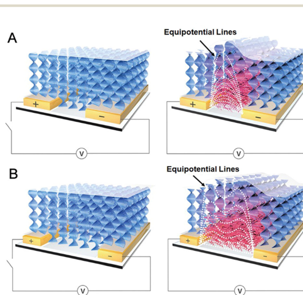
Fig. 4 Internal responding mechanism of horizontally aligned fluorinated CLCP coating above the transparent interdigitated comb-shape ITO electrode under an applied DC electric field: ideal (A) and actual model (B).
