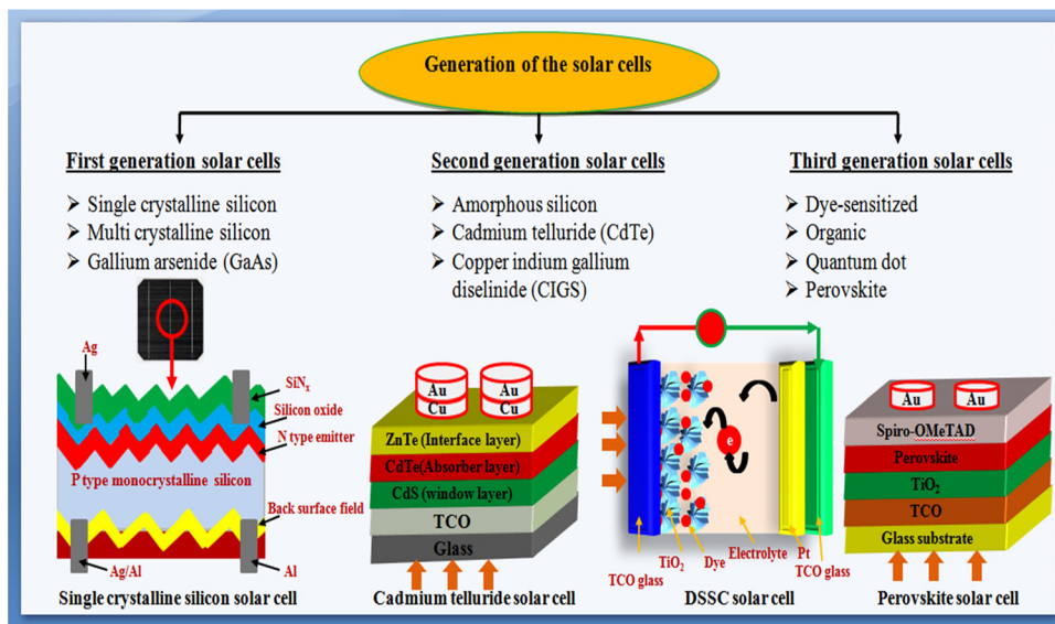
Fig. 2 Classification of solar cells based on their generation.
