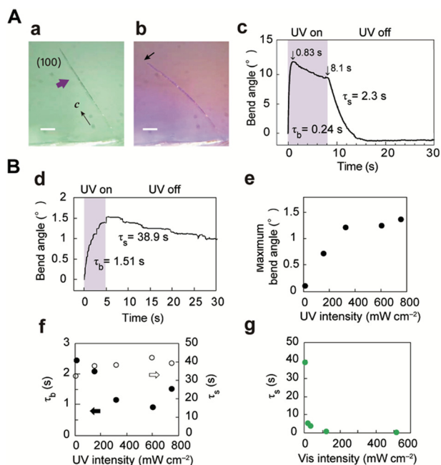
Fig. 3 Bending of thin enol- 1a crystals ((A) 385 \times 30 \times 3.8 \mu\text{m}^3 , Movie S1, (ESI†) (B) 1980 \times 67.5 \times 31.4 \mu\text{m}^3 , Movie S2, ESI†) by photoisomerisation upon UV laser irradiation. Photographs of the crystal (a) before and (b) under UV irradiation. Scale bars: 50 \mu\text{m} . (c and d) Time profile of the bend angle. (e and f) UV light intensity dependence of the (e) maximum bend angle and (f) time constants for bending (solid circles) and straightening (open circles). (g) Visible light intensity dependence of the straightening time constant.
