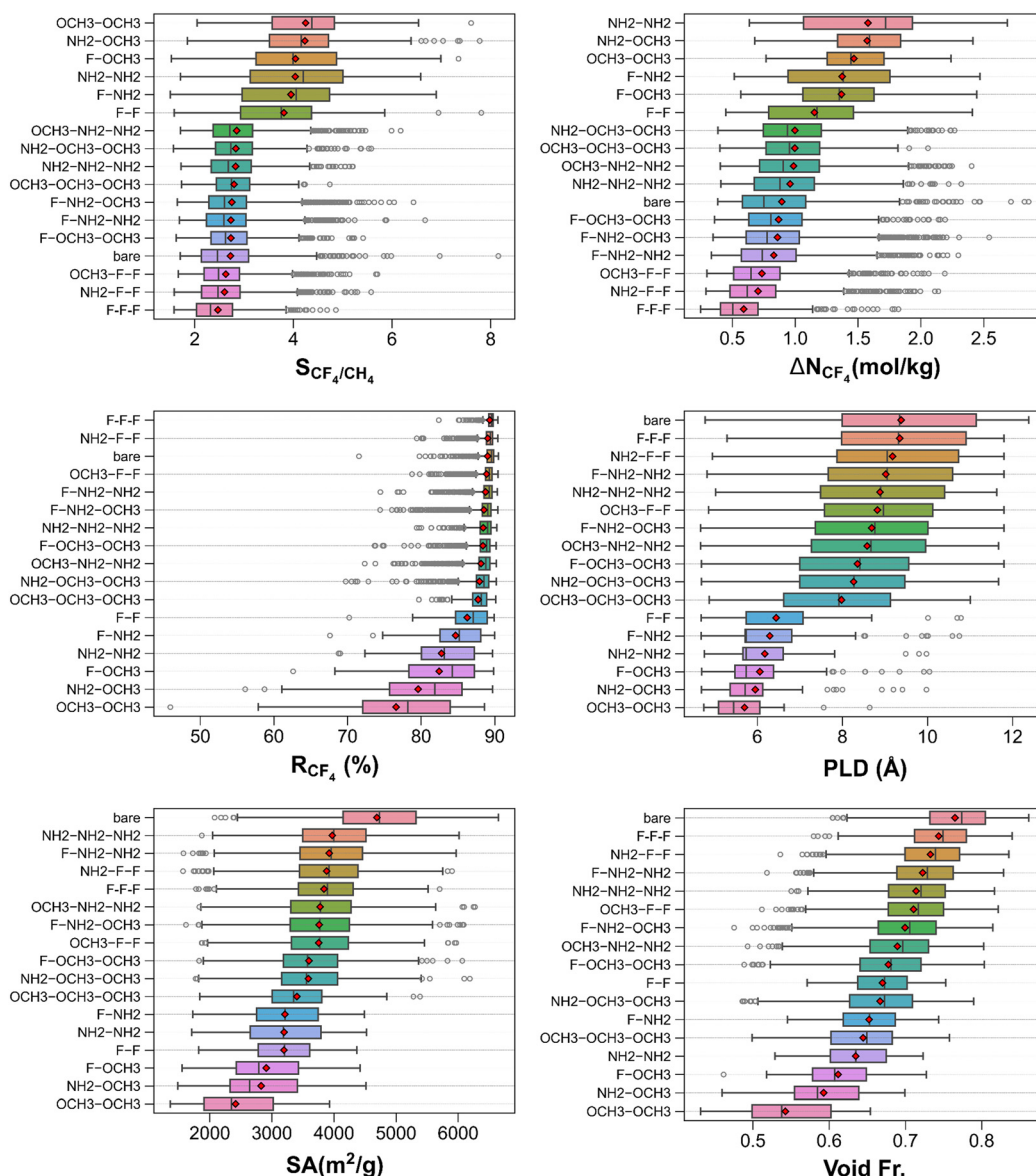
Fig. 3 CF 4 /CH 4 separation performance metrics of MTV MOFs and their pore features categorized by their functional groups. In all box-and-whisker plots, MOF groups are sorted from top to bottom by descending order where mean values are shown with red diamonds. Boxes show the range of values between the first and third quartile while the whiskers designate the distribution of other data points except outliers. Outliers are denoted as empty circles which are defined as data points away from either end of the boxes by more than 1.5 interquartile range.
