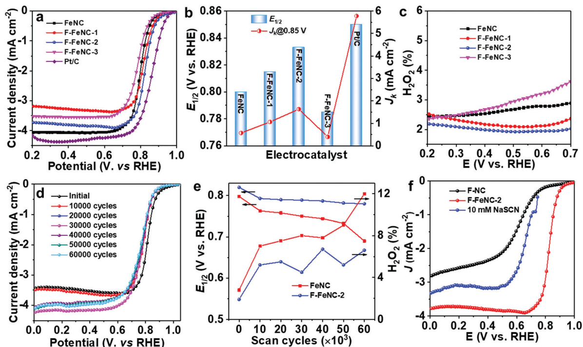
Fig. 4 (a) Steady-state ORR polarization plots recorded with a rotation speed of 900 r.p.m. and a scan rate of 5 mV s -1 , (b) J_k at 0.85 V and E_{1/2} and (c) calculated H 2 O 2 yield for FeNC, F-FeNC-1, F-FeNC-2, F-FeNC-3, and commercial Pt/C catalysts, (d) ORR polarization plots of the F-FeNC-2 and (e) the changes of E_{1/2} and H 2 O 2 yield for FeNC and F-FeNC catalysts during the durability tests. (f) ORR polarization curves of F-NC and F-FeNC and results of poisoning test with SCN - of F-FeNC.
