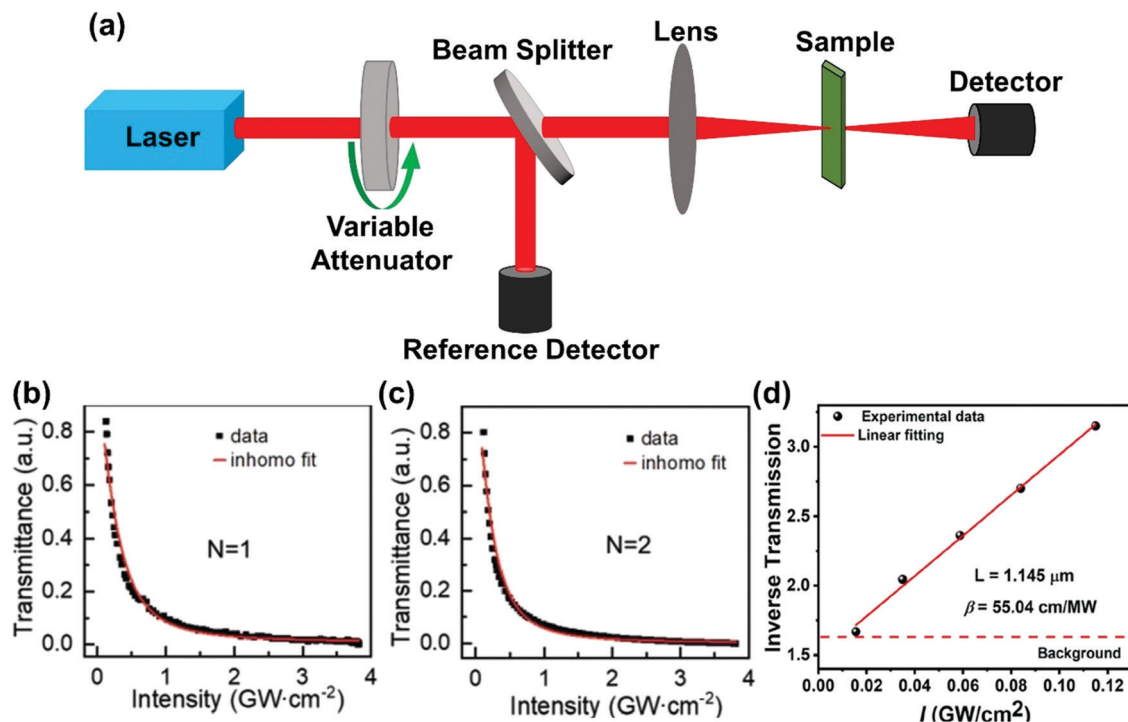
Fig. 5 (a) The schematic diagram of nonlinear transmittance technique. (b) and (c) Nonlinear transmittance versus peak intensity of the incident laser for (n-C_4H_9NH_3)_2PbI_4 ( n = 1 ) and (n-C_4H_9NH_3)_2MAPb_2I_7 ( n = 2 ) plates, respectively. (d) Inverse transmittance versus incident laser peak intensity for (R-BPEA)_2PbI_4 ( R-BPEA = (R)-1-(4-bromophenyl)ethylammonium ). (b) and (c) Reprinted with permission from ref. 70. Copyright 2019 Wiley-VCH Verlag GmbH & Co. KGaA, Weinheim. (d) Reprinted with permission from ref. 71. Copyright 2021 American Chemical Society.
