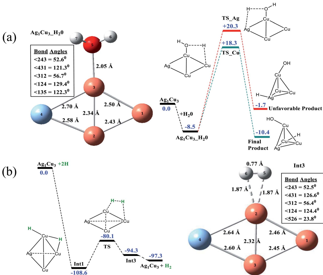
Fig. 4 (a) Left: optimized model of water bound to Cu3 of Ag_1Cu_3 with the bond parameters. Right: free energy pathway showing water splitting with relative \Delta G values (in kcal mol -1 ). (b) Right: optimized model of Int3 ( H_2 bound to Cu2 of Ag_1Cu_3 ) with the bond parameters, left: free energy pathway showing H_2 evolution with relative \Delta G values (in kcal mol -1 ).
