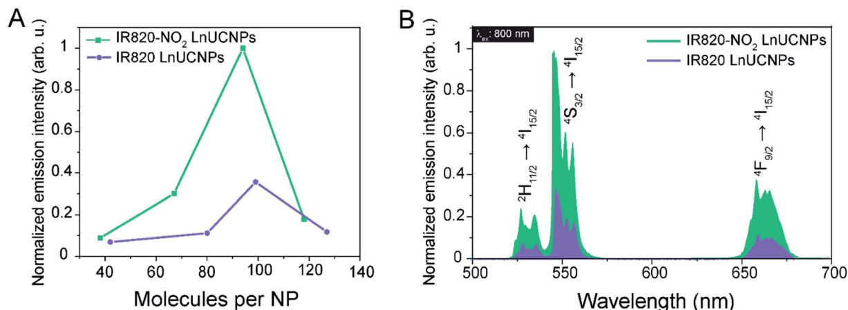
Fig. 2 (A) Integrated emission intensities of the ^4S_{3/2} \rightarrow ^4I_{15/2} transition of colloidal dispersions of IR820-NO 2 -NPs (green) and IR820-NPs (blue) as a function of the number of dye molecules per nanoparticle. (B) Upconversion emission spectra of IR820-NO 2 -NPs (green) and IR820-NPs (blue) with the optimum number of dye molecules per nanoparticle.
