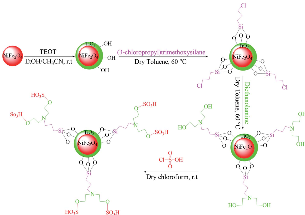
Fig. 7 Approach for the preparation of the \text{NiFe}_2\text{O}_4@\text{TiO}_2\text{-SiO}_2\text{-Pr-DEA-OSO}_3\text{H} nanocatalyst (r.t: room temperature). This figure was adapted with permission from Chem. Sel. , 2019, 4, 17–23. 71
