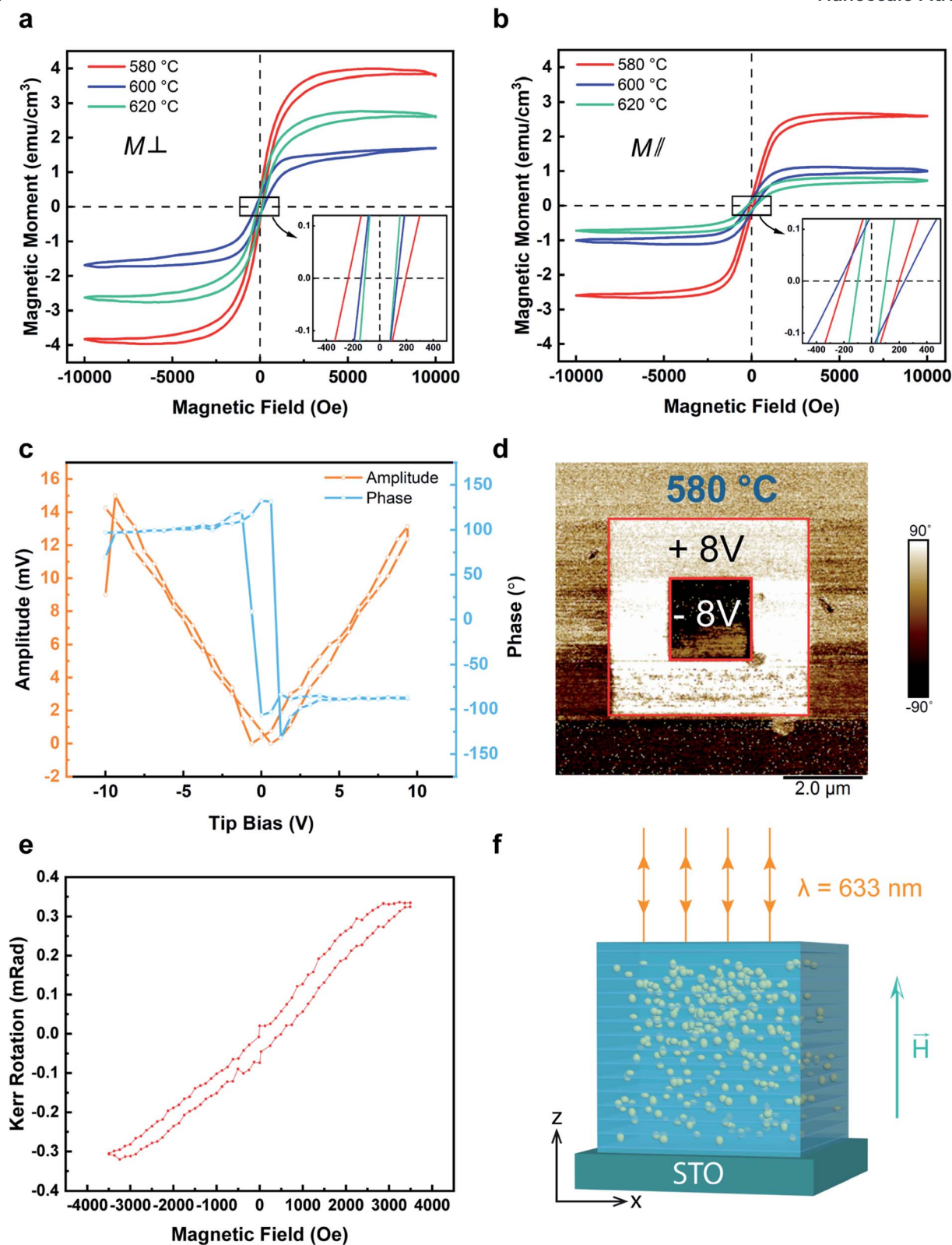
Fig. 5 Multiferroic properties of the BAMO-Au system. (a) and (b) Ferromagnetic response of BAMO-Au thin films along out-of-plane and in-plane directions, respectively. The insets are the enlarged center area of the ferromagnetic hysteresis loop showing the coercive field. (c) Amplitude and phase switching behavior as a function of tip bias for the BAMO-Au thin film grown at 580 °C. (d) Vertical PFM phase map for the BAMO-Au thin film grown at 580 °C, obtained by poling with +8 V (bright contrast) over 5 \times 5 \mu\text{m}^2 and -8 V (dark contrast) over 2 \times 2 \mu\text{m}^2 . The outer area is not poled with voltage, and therefore has a random inherent phase. (e) Polar MOKE measurements for BAMO-Au films deposited at 580 °C. The magnetic field is applied along the out-of-plane direction. The hysteresis loop shows the magneto-optical coupling effect. (f) The experimental configuration for Polar MOKE measurements. The magnetic field is applied along the out of plane direction. The wavelength of the applied laser is about 630 nm.
