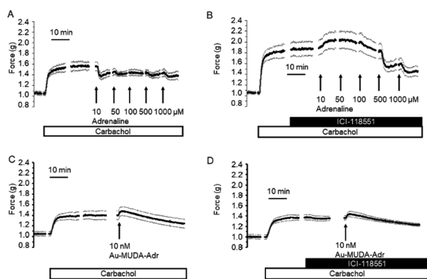
Fig. 6 Concentration-dependent relaxation of segments from rat upper respiratory tract by adrenaline; ( 10\text{--}1000 \mu\text{mol l}^{-1} ; arrows) under control conditions (A) and after pretreatment (B) with the \beta_2 -blocker ICI-118551 ( 10 \mu\text{mol l}^{-1} ; black bar). Missing effect of Au-MUDA-ADR ( 10 \text{nmol l}^{-1} ; arrows) under control conditions (C) or after pretreatment (D) with ICI-118551 ( 10 \mu\text{mol l}^{-1} ; black bar). All segments were precontracted with the cholinergic agonist carbachol ( 0.5 \mu\text{mol l}^{-1} ; white bar). Data are means (thick line) \pm SEM (dotted lines), n = 5\text{--}8 .
