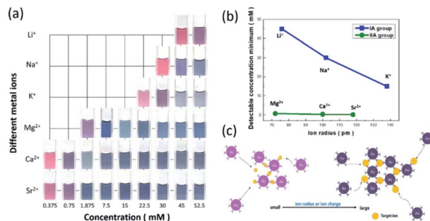
Fig. 5 (a) Comparative colorimetric examinations of AuNP probes for detecting various cation ions. (b) Plot of the detectable concentration minimum of various cation ions with respect to the corresponding ion radii. (c) Illustrated detection mechanism of AuNP probes influenced by ion radius and charge of target analytes.
