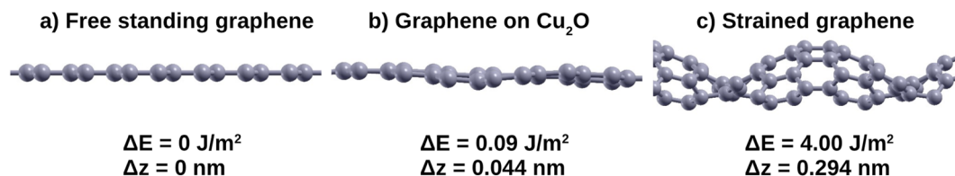
Fig. 6 DFT results for the geometries, surface energies and out-of-plane deformations of graphene with three different curvatures. (a) Flat, free-standing graphene, (b) mildly curved graphene on \text{Cu}_2\text{O}(111) and (c) free-standing graphene with a strong curvature, imposed by a 19% lateral compression. The surface energies are expressed as the difference with respect to the value for the free-standing graphene layer.
