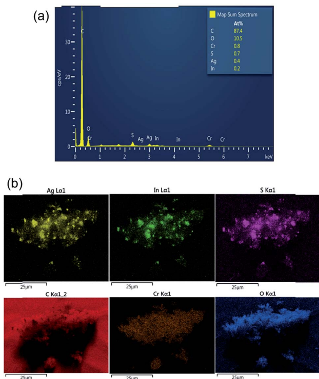
Fig. 7 (a) EDS pattern and (b) EDX elemental mapping of 40% AIS@MIL-101(Cr) nanocomposites.
