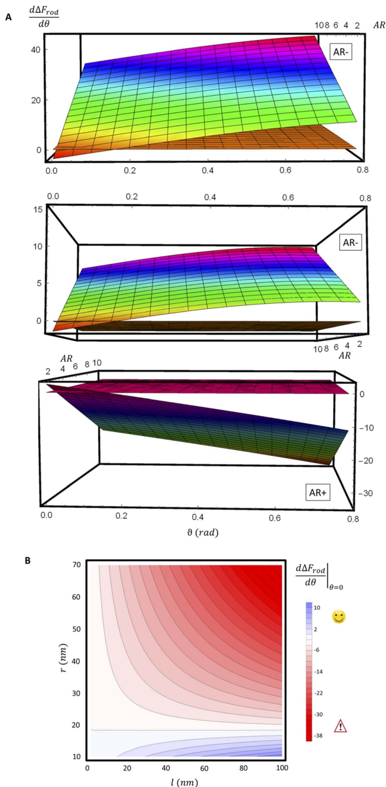
Fig. 8 (A) Derivative of \Delta F_{rod} with respect to \theta , as a function of \theta and of the aspect ratio AR. Typical values of 0.002k_B T/\text{nm}^2 and 2.3k_B T , respectively, were used for \varepsilon and \kappa . The plots correspond to three values of r : 20 nm (top), and 40 nm (middle) – which are smaller than r^* , and 60 nm (bottom) which is larger than r^* ; a flip from AR– to AR+ is observed between these two regimes. For a clearer view the zero plane was added to the surface plots as a reference. (B) \frac{d\Delta F_{rod}}{d\theta} \Big|_{\theta=0} is shown as a function of r and of l . Blue color represents positive values, which indicate on vanishing uptake and higher safety of the rods, and the red color represent negative values and increased probability for cytotoxicity. A threshold in r^* \sim 18 nm, at which the system switches from AR– to AR+ is observed.
