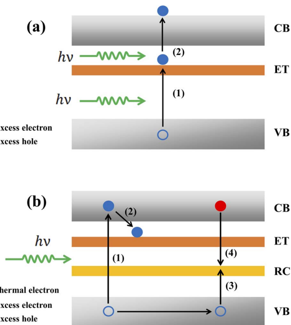
Fig. 8 Schematic band diagrams showing transitions involving the (a) PPC mechanism for In 0.35 Al 0.65 N NRs and (b) NPC mechanism for In 0.57 Al 0.43 N and In 0.68 Al 0.32 N NRs. CB denotes the conduction band. VB denotes the valence band. ET denotes electron trap states. RC denotes recombination centers.
