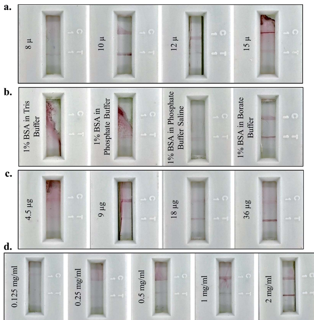
Fig. 3 Optimization of LFA fabrication: (a) optimisation of various pore sizes of the NC membrane ( 8\ \mu\text{m} , 10\ \mu\text{m} , 12\ \mu\text{m} , and 15\ \mu\text{m} ) for the ease of flow; (b) selection of ideal blocking buffer i.e. BSA in Tris buffer, phosphate buffer, phosphate buffer saline or borate buffer, to prevent non-specific binding of the NC membrane; (c) variable concentration of the JEV NS1 Ab for conjugation with AuNPs ( 4.5\ \mu\text{g} , 9\ \mu\text{g} , 18\ \mu\text{g} and 36\ \mu\text{g} ); (d) different concentrations of the JEV NS1 Ab ( 0.125\ \text{mg ml}^{-1} , 0.25\ \text{mg ml}^{-1} , 0.5\ \text{mg ml}^{-1} , 1\ \text{mg ml}^{-1} and 2\ \text{mg ml}^{-1} ) for test line coating on the NC membrane.
