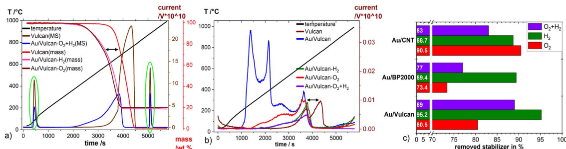
Fig. 4 (a) TG-MS measurements with currents normalized to the CO 2 ( m/z = 44u ) peak area, baseline corrected, (b) SO 2 ( m/z = 64u ) currents multiplied \times 1000 , green circles in (a) CO 2 injections for normalization, (c) amount (as noted at base of the bars) of removed stabilizer from AuNP by the different treatments (see text).
