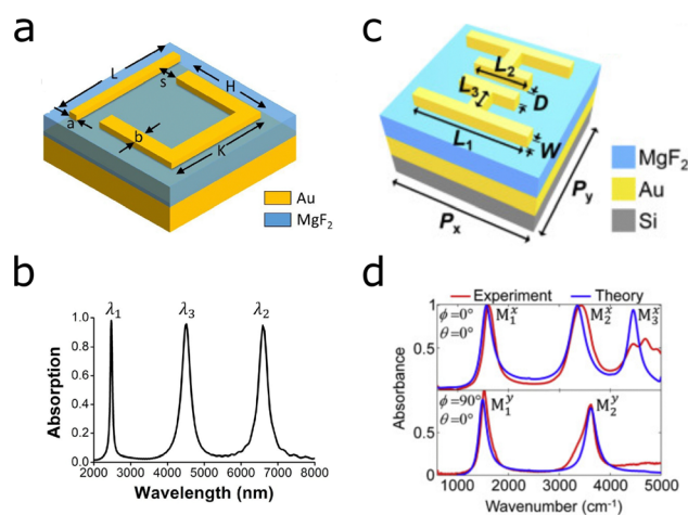
Fig. 13 Multi- and dual-band perfect absorbers based on gold nanostructures. The designs are constructed on gold mirrors and MgF 2 dielectric spacers. (a) Geometry of the nanobar and U-shaped antenna design. (b) Plasmonic response of the structure a, with \lambda_1 , \lambda_2 and \lambda_3 corresponding to H, L and K, respectively. Reprinted from ref. 120 with permission from Elsevier. (c) Multi-band perfect absorber based on a mirrored asymmetric double H. (d) (top) Parallel illumination plasmonic response of structure e, with \lambda_1 and \lambda_2 and \lambda_3 corresponding long and short antennas, and the space between these two, respectively. (bottom) In perpendicular polarization the modes arise from dipolar and quadrupolar coupling between the two mirrored asymmetric H-shapes. Reprinted from ref. 126 with permission from Elsevier.
