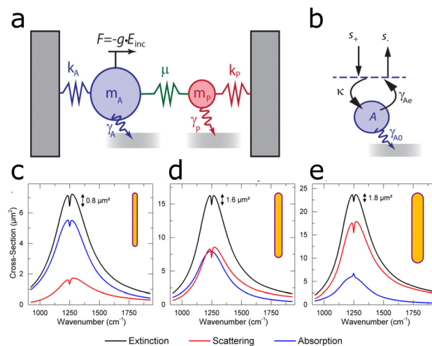
Fig. 3 (a) Schematic view of a damped harmonic oscillator consisting of a bright (A) and a dark (P) mode. The external radiation drives the bright mode A via a force g \times E_{inc} . The dark mode P does not interact with the external field but is indirectly driven by coupling with mode A via a driving rate, \mu . The bright mode A experiences a larger damping, \gamma_A , than the dark mode, \gamma_P . (b) Schematic illustration of a cavity in the temporal coupled mode theory. Reprinted with permission from ref. 64. Copyright 2013 American Chemical Society. (c) Extinction (black), absorption (blue), and scattering (red) of a dominantly absorbing antenna enhancing the IR signal (d) of a critically coupled antenna (scattering and absorption approximately equal) and (e) of a dominantly scattering antenna enhancing signal. Adapted with permission from ref. 53. Copyright 2015 American Chemical Society.
