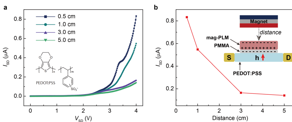
Fig. 6 Switching on a transistor with the mag-PLM. (a) Source to drain current–voltage characteristics of a PEDOT:PSS transistor in which the mag-PLM is used as the electrolyte gate. As the magnet approaches the mag-PLM, the current has increased. (b) Distance-dependent source to drain current. The inset shows the scheme of the device.
