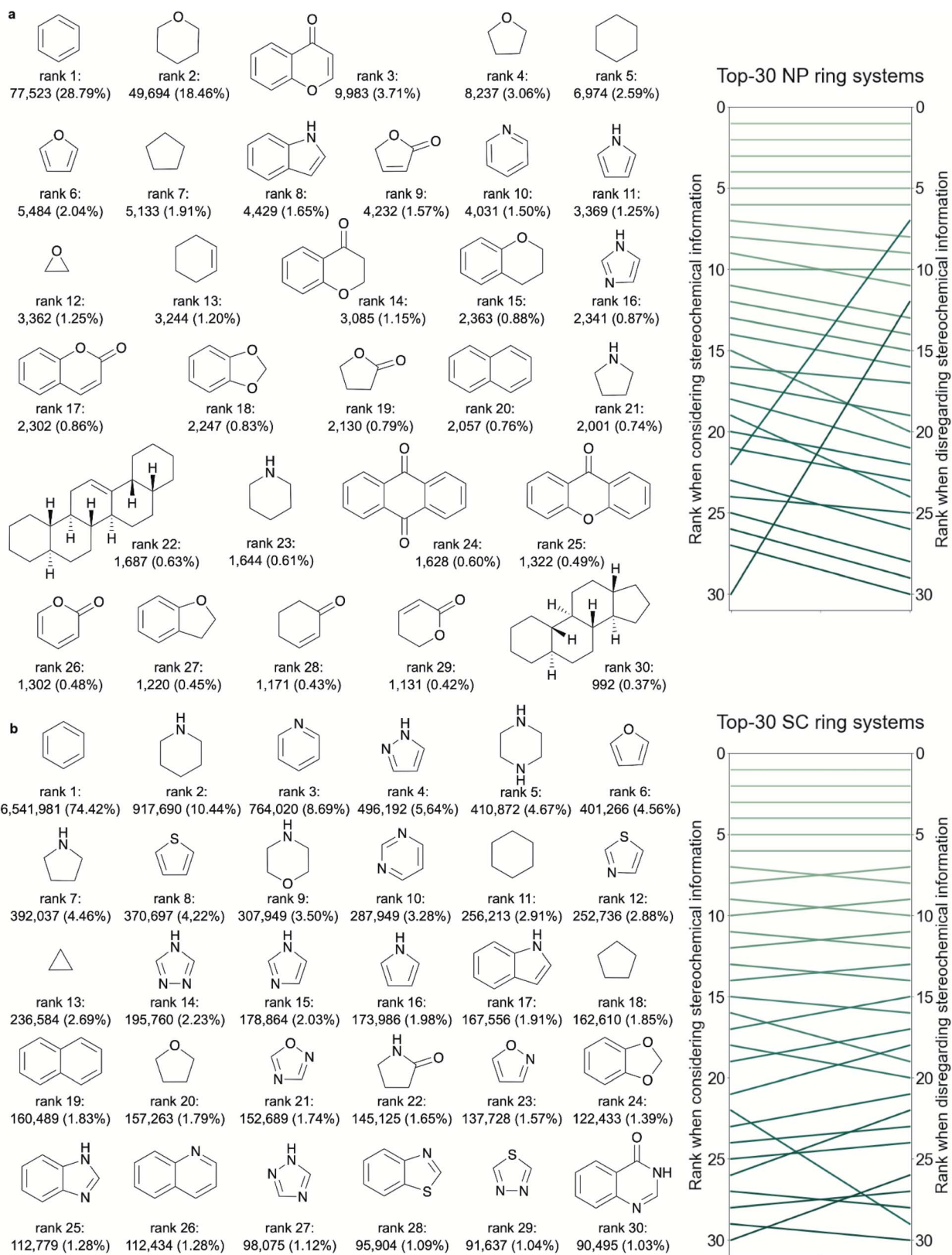
Fig. 2 Occurrences (absolute numbers and percentages) of the 30 most frequent ring systems in (a) NPs and (b) SCs. The molecular structures are sorted by decreasing frequency, taking into account stereochemical information. The diagrams on the right of each panel compare the ranks of these ring systems when considering stereochemical information (left) and when disregarding it (right). Note that, for the sake of clarity, lines connecting to ranks exceeding 30 are not depicted. For example, in (a) the line connecting rank 28 on the left to rank 33 on the right is not shown.
