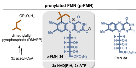
Fig. 5 Summary of prenylated flavin mononucleotide biosynthesis with building blocks marked in sienna and blue including positions where they end up in prenylated flavin mononucleotide (prFMN) 36 . Coenzyme-dependent enzymes (refer to the synthesis of DMAPP by the mevalonate pathway): NAD(P)H: HMG-CoA reductase; ATP: mevalonate kinase and phosphomevalonate kinase.
