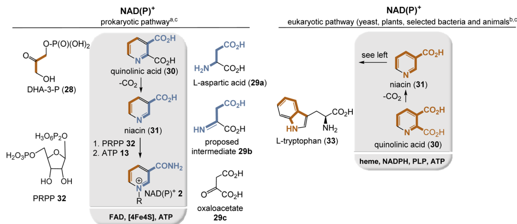
Fig. 3 Summary of NAD + biosyntheses in prokaryotes and plants: building blocks are marked in sienna and blue including positions where they end up in quinolinic acid ( 30 ), niacin ( 31 ) and finally in NAD(P) + 2. a Coenzyme-dependent enzymes (bacteria, archaea): FAD: L-aspartate oxidase (NadB); Fe 4 S 4 : quinolinate synthetase (NadA). b Coenzyme-dependent enzymes (eukaryotes): heme: tryptophan 2,3-dioxygenase (TDO); NADPH: kynurenine 3-monooxygenase (KMO); PLP: kynureninase (KYN); Fe II : 3-hydroxyanthranilate-3,4-dioxygenase (HAD). c Both pathways: ATP for transformation of NAD + to NAD(P) + .
