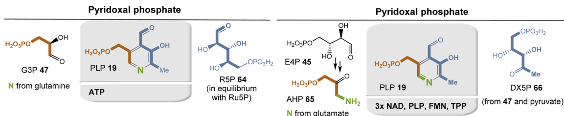
Fig. 26 Summary of pyridoxal phosphate biosynthesis: building blocks are marked in sienna, blue and green at positions where they end up in PLP 19. Coenzyme-dependent enzymes (left): ATP: glutamine synthase. Coenzyme-dependent enzymes (right): NAD + : erythrose-4-phosphate dehydrogenase; NAD + : erythronate-4-phosphate dehydrogenase; NAD + : 4-hydroxythreonine-4-phosphate dehydrogenase; PLP: phosphoserine aminotransferase; FMN: pyridoxine 5'-phosphate oxidase; TPP: 1-deoxyxylulose 5-phosphate synthase.
