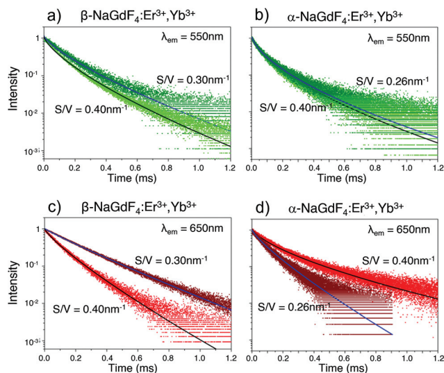
Fig. 7 UC luminescence decay curves for (a), (c) \beta - and (b), (d) \alpha - \text{NaGdF}_4 UCNPs of two different sizes ( S/V as labeled in the figure) dispersed in toluene monitoring either the UCNPs' green ( \lambda_{\text{em}} = 550 \text{ nm} ) or red ( \lambda_{\text{em}} = 650 \text{ nm} ) emission following 980 nm excitation. From these decay curves, respective excited state lifetimes have been determined using a Kohlrausch fitting function (solid lines).
