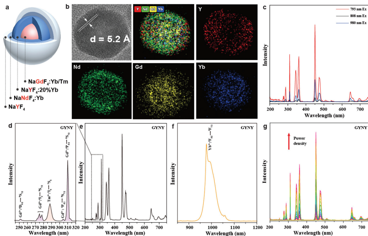
Fig. 1 (a) Schematic illustration of a \text{NaGdF}_4:49\%\text{Yb},1\%\text{Tm}@NaYF_4:20\%\text{Yb}@NaNdF_4:10\%\text{Yb}@NaYF_4 (GYNY) nanoparticle. (b) High-resolution TEM image and elemental mapping of the corresponding GYNY nanocrystal. (c) Corresponding upconversion luminescence spectra of GYNY nanoparticles in cyclohexane under 793, 808 and 980 nm excitation at a power density of 28.0 \text{ W cm}^{-2} . (d–f) Room-temperature luminescence spectra in the range of 240–750 nm and 850–1200 nm of GYNY nanoparticles in cyclohexane. (g) Excitation-power-dependent upconversion emission spectra of GYNY nanoparticles under 793 nm excitation.
