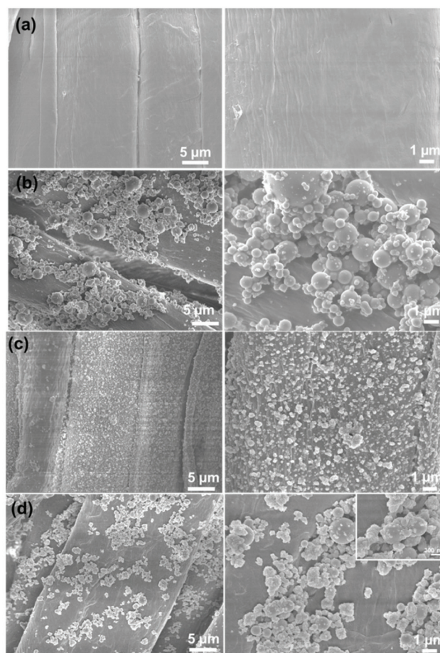
Fig. 2 SEM images of (a) pristine cotton fabric, (b) SiO 2 /PDMS-coated cotton fabric, (c) TiO 2 /PDMS-coated cotton textile, and (d) SiO 2 -TiO 2 /PDMS-coated cotton fabric.
