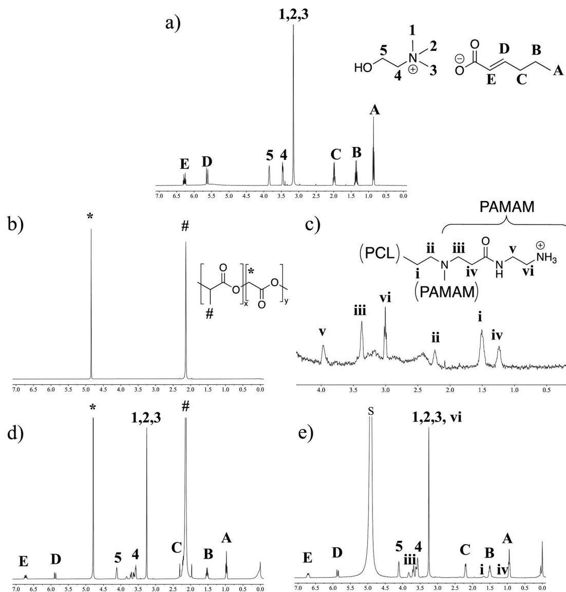
Fig. 2 1 H-NMR shows different chemical composition of the IL layering in PLGA NPs compared to LDBC NPs. (a) 1 H NMR of choline and trans -2-hexenoic acid [1:1]. (b) PLGA NPs, (c) LDBC NPs, (d) IL-PLGA NPs, and (e) IL-LDBC NPs. (d) and (e) include 25 \mu L [TMS]/700 \mu L [NPs in D 2 O] for IL quantification.
