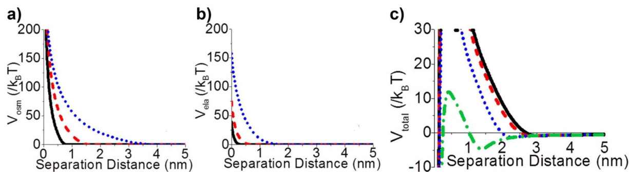
Fig. 4 Effect of ligand thickness at t = 0.4 (solid black line), 0.8 (red dashed line), and 2.0 (blue dotted line) nm on the (a) osmotic ( V_{osc} ) and (b) elastic ( V_{el} ) interaction potentials as a function of edge-to-edge separation distances between two NPs. (c) Effect of ligand tilt angle, 0 (solid black line), 20 (red dashed line), 40 (blue dotted line), and 60^\circ (green dashed and dotted line), on the total potential of a NPs pair functionalized. Adapted with permission from ref. 70 (copyright 2015, American Chemical Society).
