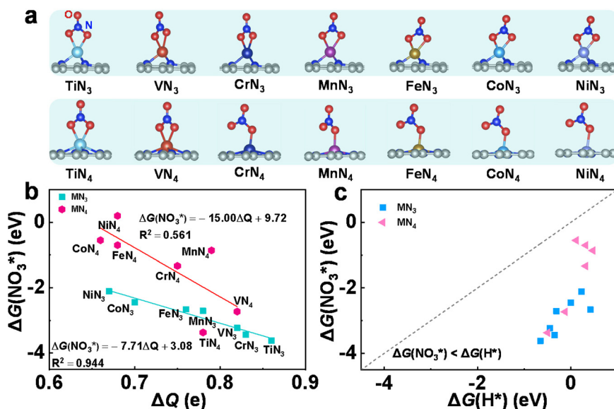
Fig. 2 (a) Atomic configurations of the \text{TMN}_3 @G (upper panel) and \text{TMN}_4 @G (lower panel) with the adsorbed \text{NO}_3^- . (b) The relationship between charge transfer ( \Delta Q ) of the \text{NO}_3^- and its binding free energy ( \Delta G(\text{NO}_3^*) ). (c) Comparison of the binding free energies of \text{NO}_3^- ( \Delta G(\text{NO}_3^*) ) and H atom ( \Delta G(\text{H}^*) ).
