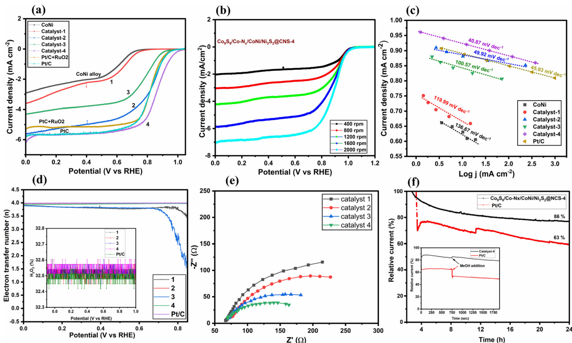
Fig. 6 Electrochemical ORR performances: (a) LSV curves of CoS/Co-N x /CoNi/NiS 2 @CNS 1–4, commercial 20% Pt/C and Pt/C + RuO 2 in O 2 -saturated 0.1 M KOH, (b) LSV curves of CoS/Co-N x /CoNi/NiS 2 @CNS-4, at various rotation rates, (c) Tafel plots of catalysts 1–4 and Pt/C, (d) Electron transfer number ( n ) of catalysts 1–4, and Pt/C, inset: the corresponding peroxide yields, (e) EIS spectra of catalysts 1–4, and (f) chronoamperometric responses of Co 9 S 8 /Co-N x /CoNi/Ni 3 S 2 @CNS-4, and commercial 20% Pt/C in O 2 -saturated 0.1 M KOH solution at a rotation rate of 1600 rpm at ~0.4 V vs. RHE.
