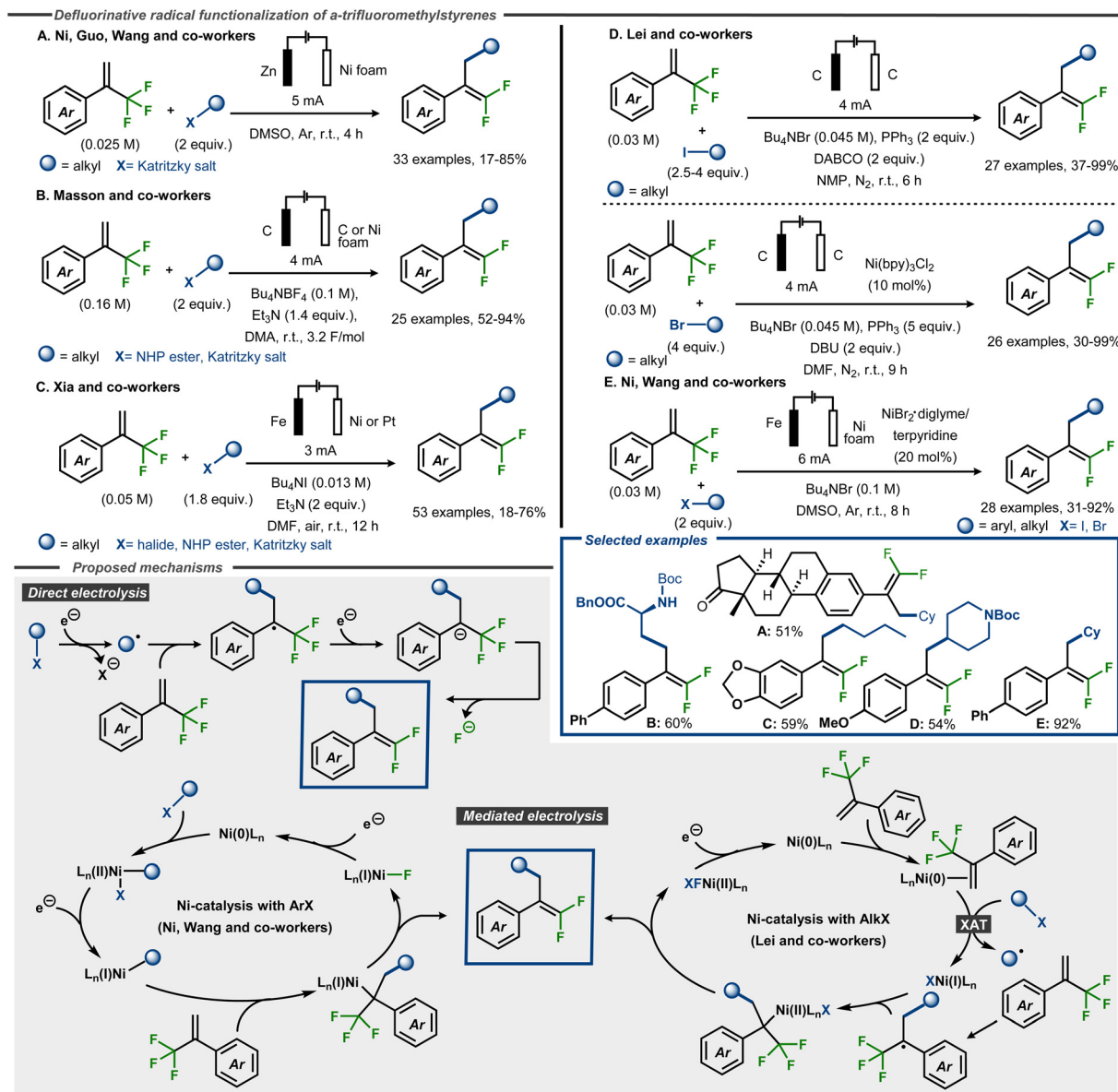
Fig. 18 Electrocatalytic formation of \gamma -functionalized gem -difluorostyrenes from \alpha -trifluoromethyl styrenes and radical precursors. 64–68
