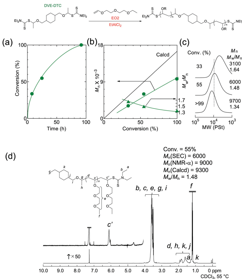
Fig. 3 Living cationic polymerization of EO2 with bifunctional dithiocarbamate (DVE-DTC): [\text{EO2}]_0/[\text{DVE-DTC}]_0/[\text{EtAlCl}_2]_0/[\text{THF}]_0 = 1000/10/15/400 mM in toluene at 0^\circ\text{C} . (a) time-conversion, (b) M_n and M_w/M_n curves, (c) SEC curves, and (d) ^1\text{H} NMR spectrum of the obtained polymer.
