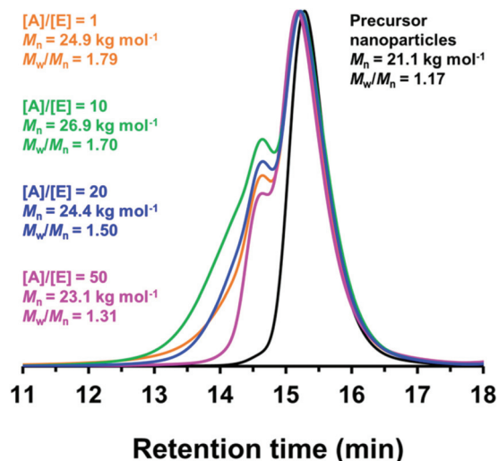
Fig. 3 GPC curves (vs. a series of near-monodisperse poly(methyl methacrylate) calibration standards) recorded using a refractive index detector for P(LMA 50 -stat-GlyMA 9 )-PMMA 67 (prepared in mineral oil at 20% w/w solids at 90 °C) (black curve) and the benzylamine-derivatized P(LMA 50 -stat-GlyMA 9 )-PMMA 67 produced when using an [amine]/[epoxy] molar ratio of 1 (orange curve), 10 (green curve), 20 (blue curve) or 50 (pink curve). A systematic reduction in M_w/M_n was observed when increasing the [amine]/[epoxy] molar ratio.
